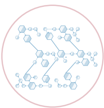
Cross-link
