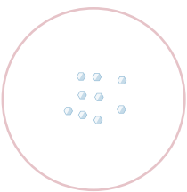
Cross-linking
